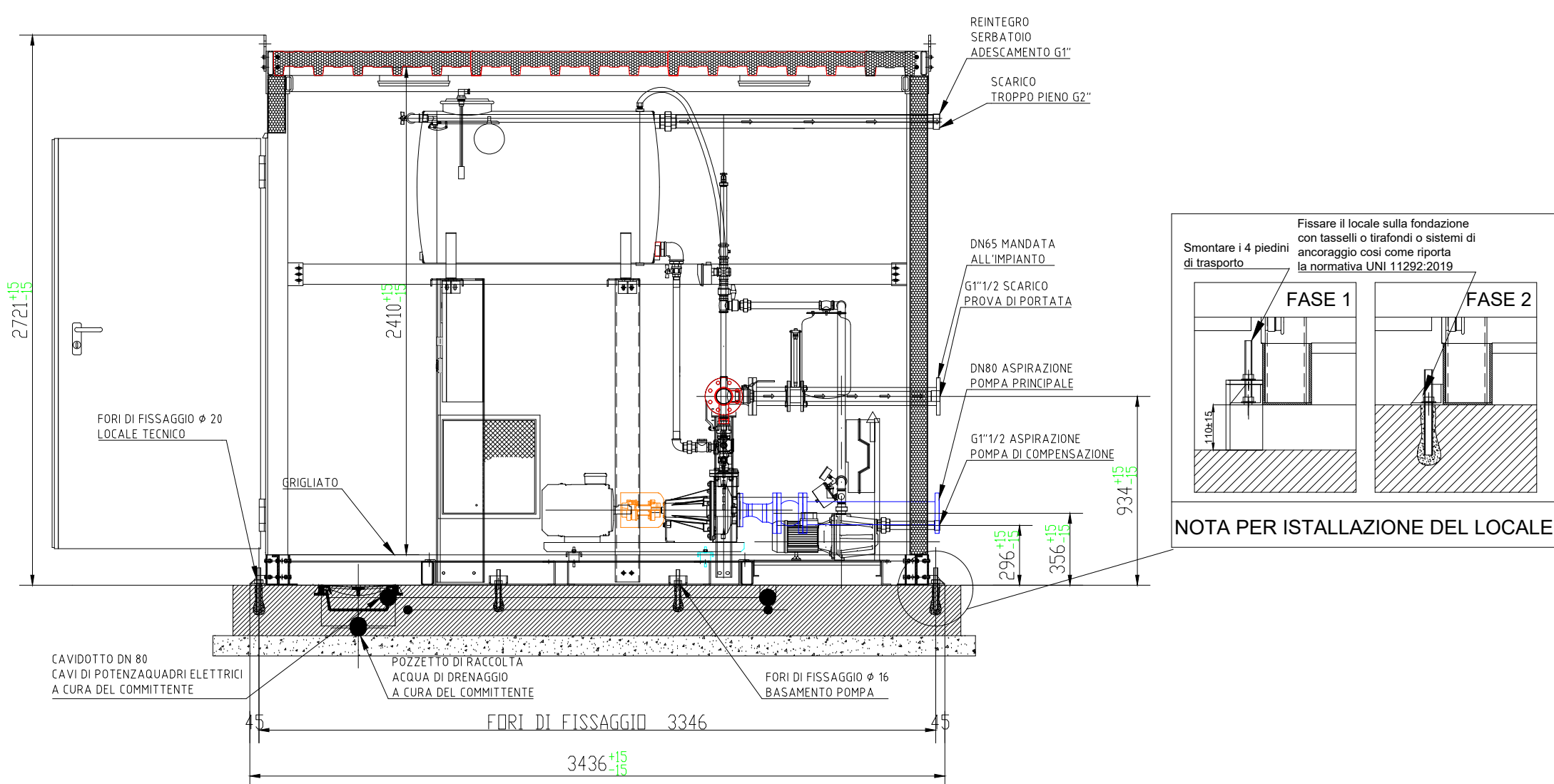
Vista Laterale / Side View
