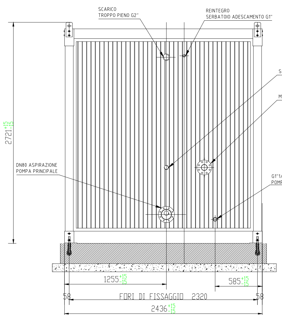
Vista Frontale / Front View
