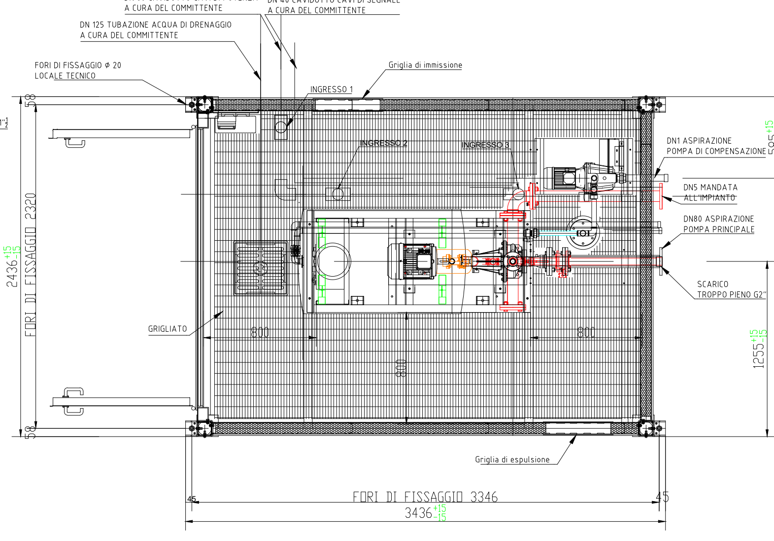
Vista Pianta / Plan View
